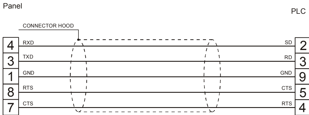
figure 1. Cable diagram
