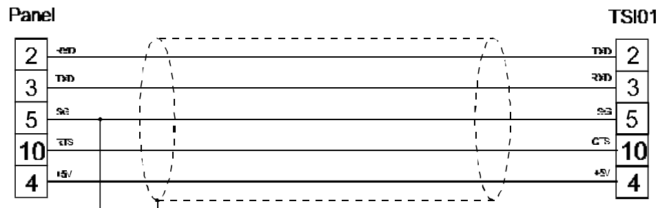
figure 1. Cable diagram
