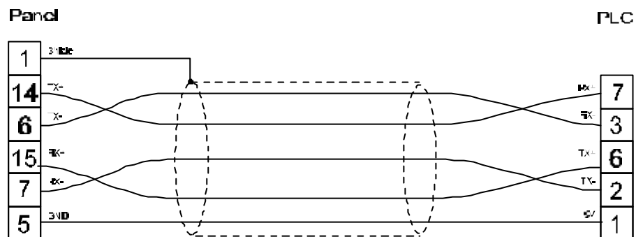
Figure 1. Cable diagram
